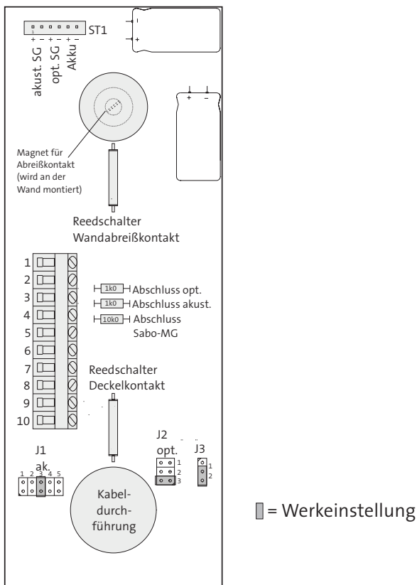
Skizze 2 (Platine)
